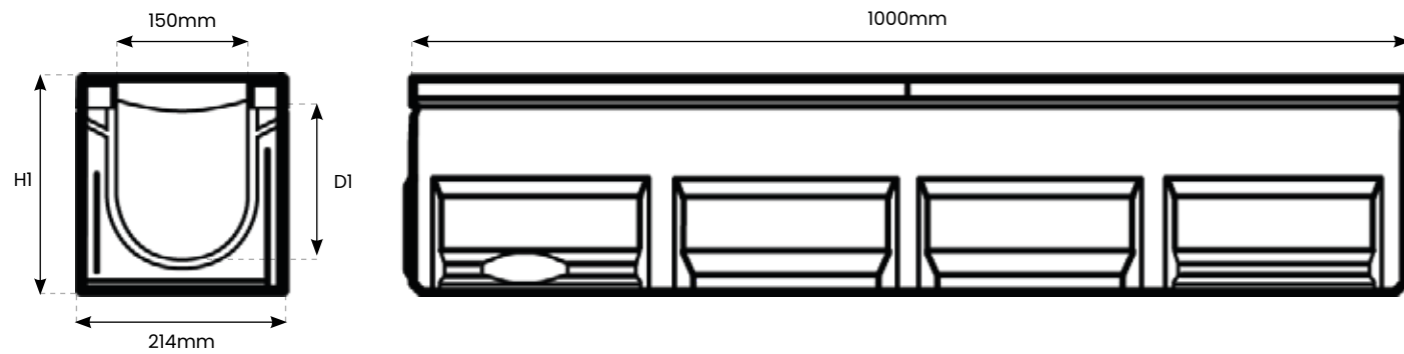
1000mm Channel Diagram
