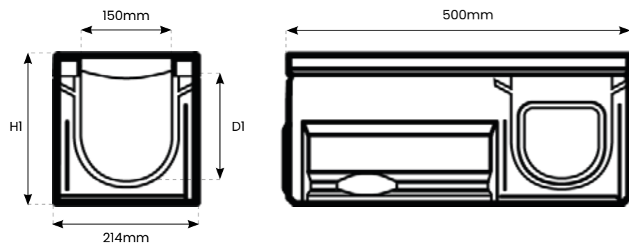
500mm Channel Diagram
