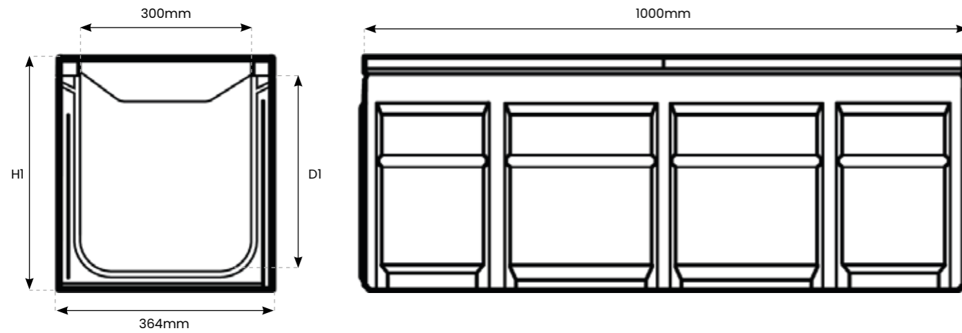
1000mm Channel Diagram
