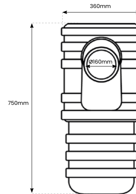
Gully Pot Diagram
