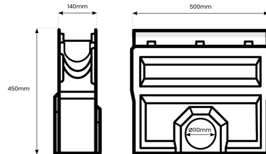
Sump Unit Diagram
