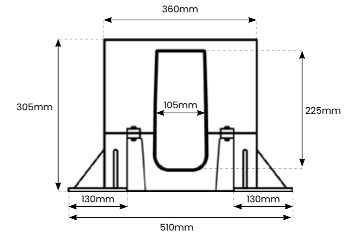
Universal Outfall Diagram
