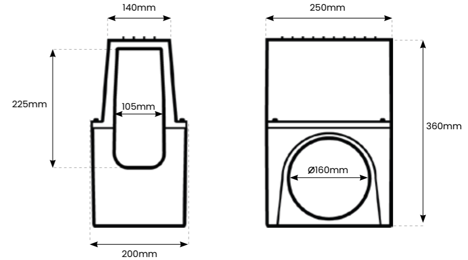
Rodding Access Unit Diagram
