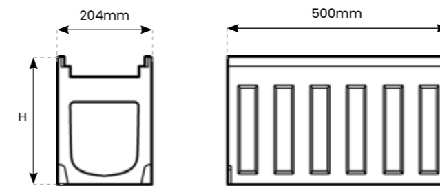
Sump Unit - Upper Part
