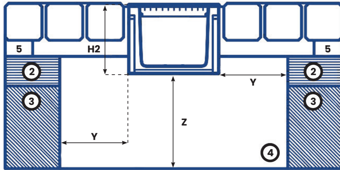
Block Paving
